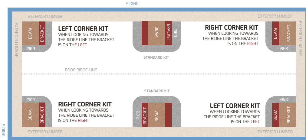
LEFT + RIGHT ARE DETERMINED FROM THE PERSPECTIVE OF LOOKING TOWARDS THE RIDGE LINE
