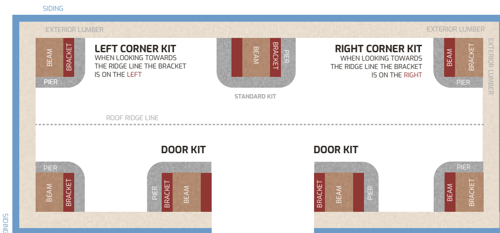
DOOR KITS USE A DIFFERENT CONCRETE PIER FORM THAN A STANDARD BRACKET THE DOOR FORMS ARE REVERSIBLE AND DON'T HAVE A LEFT RIGHT ORIENTATION
