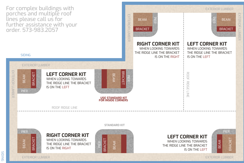
EXAMPLE OF BUMP OUT BUILDING
